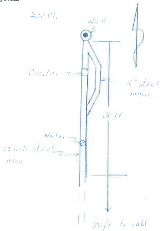
Diagram of System
