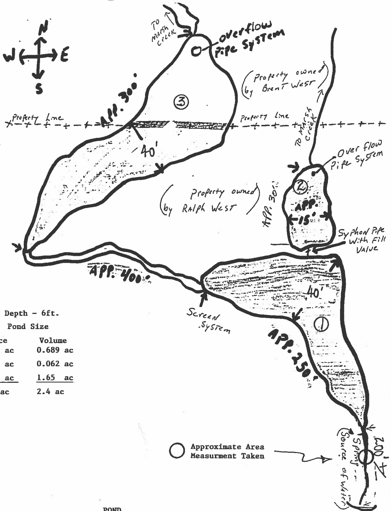
POND SCHEMATIC
