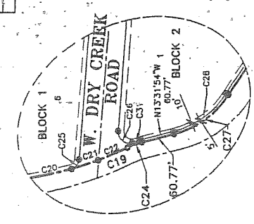
DETAIL "B"-NTS
