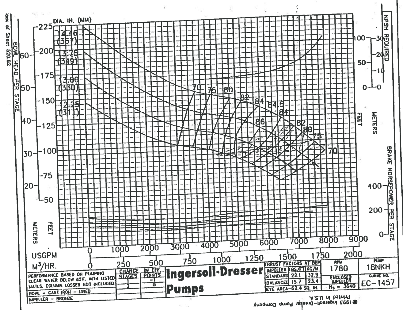
Figure 4. Pump curves for the Ingersoll-Dresser 18NKH
