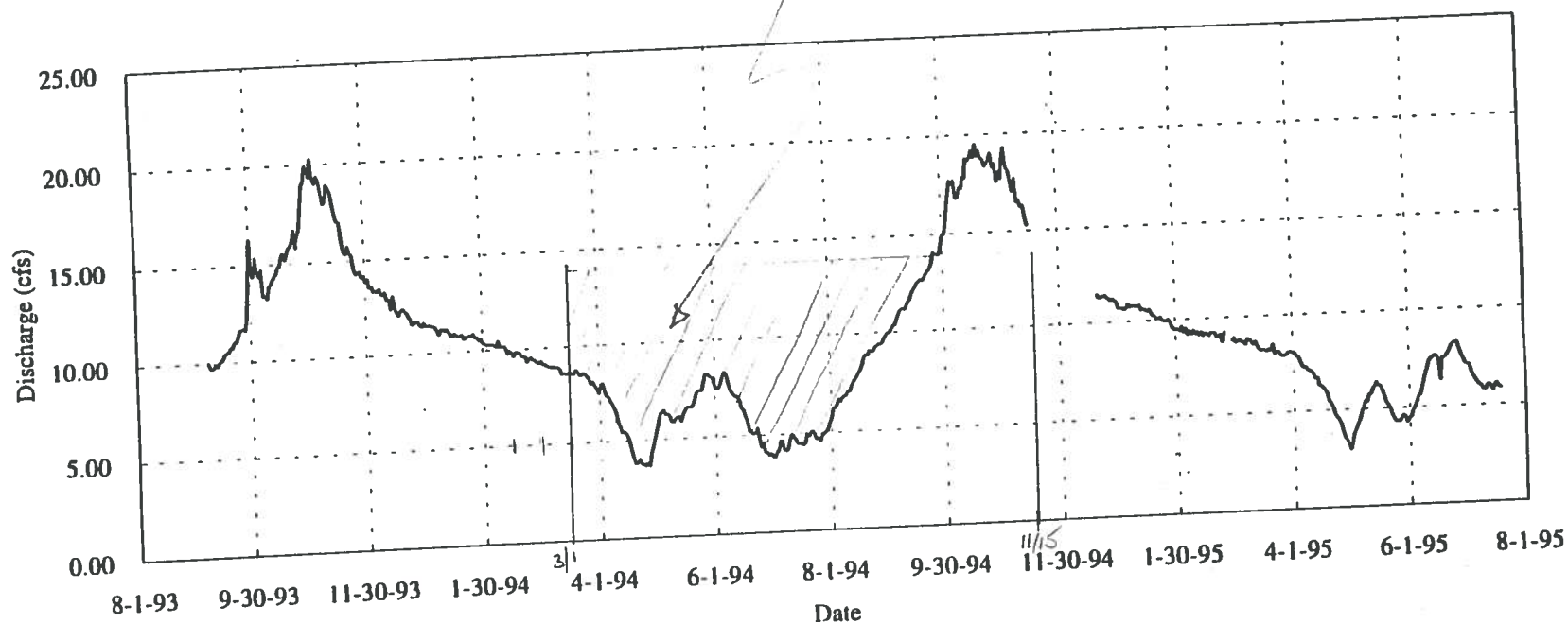
Figure 2. Measured discharge of Curren tunnel
