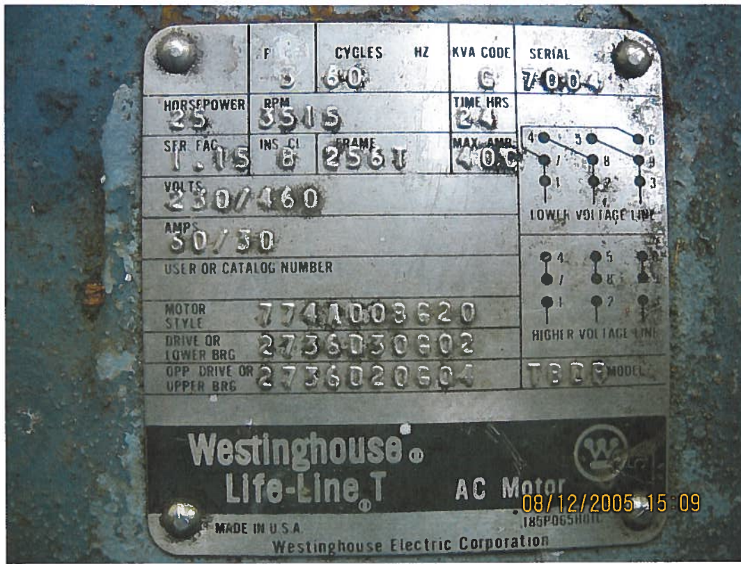
Photo 3: Motor plate.
