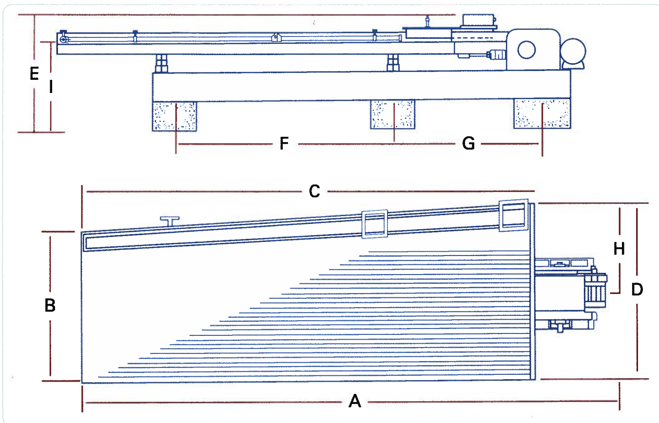
Wilfley table aerial and side view
