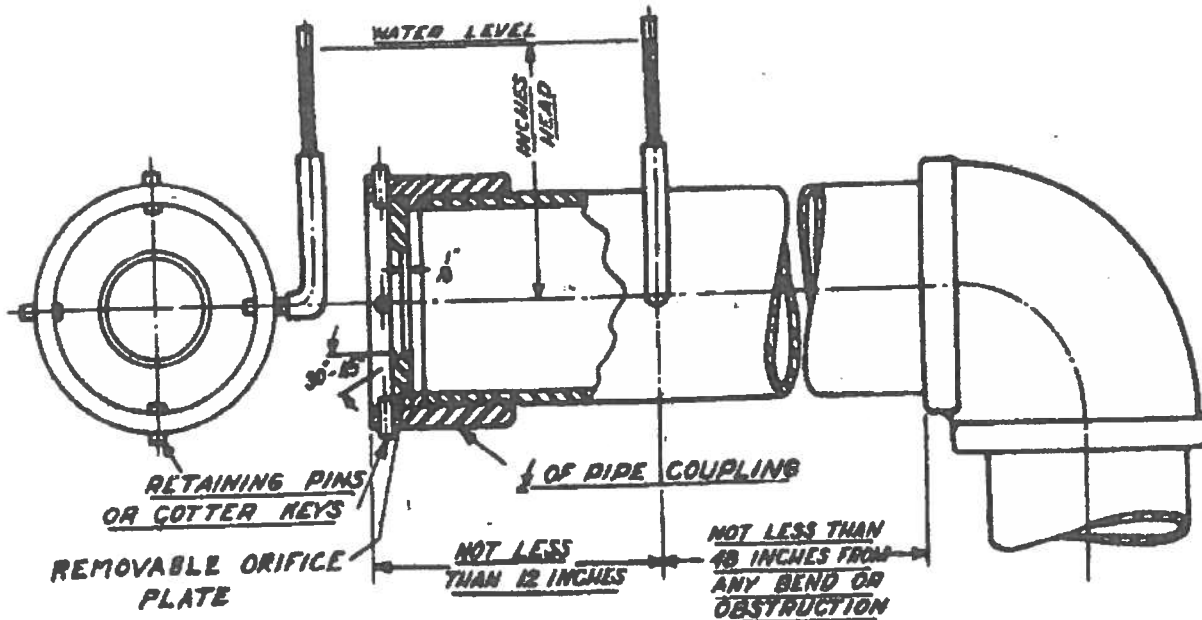
ORIFICE SET-UP
