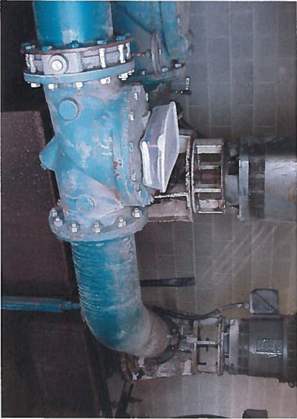
↑ Pump 1 & pump 2 with 18" pipeline to center pivots
