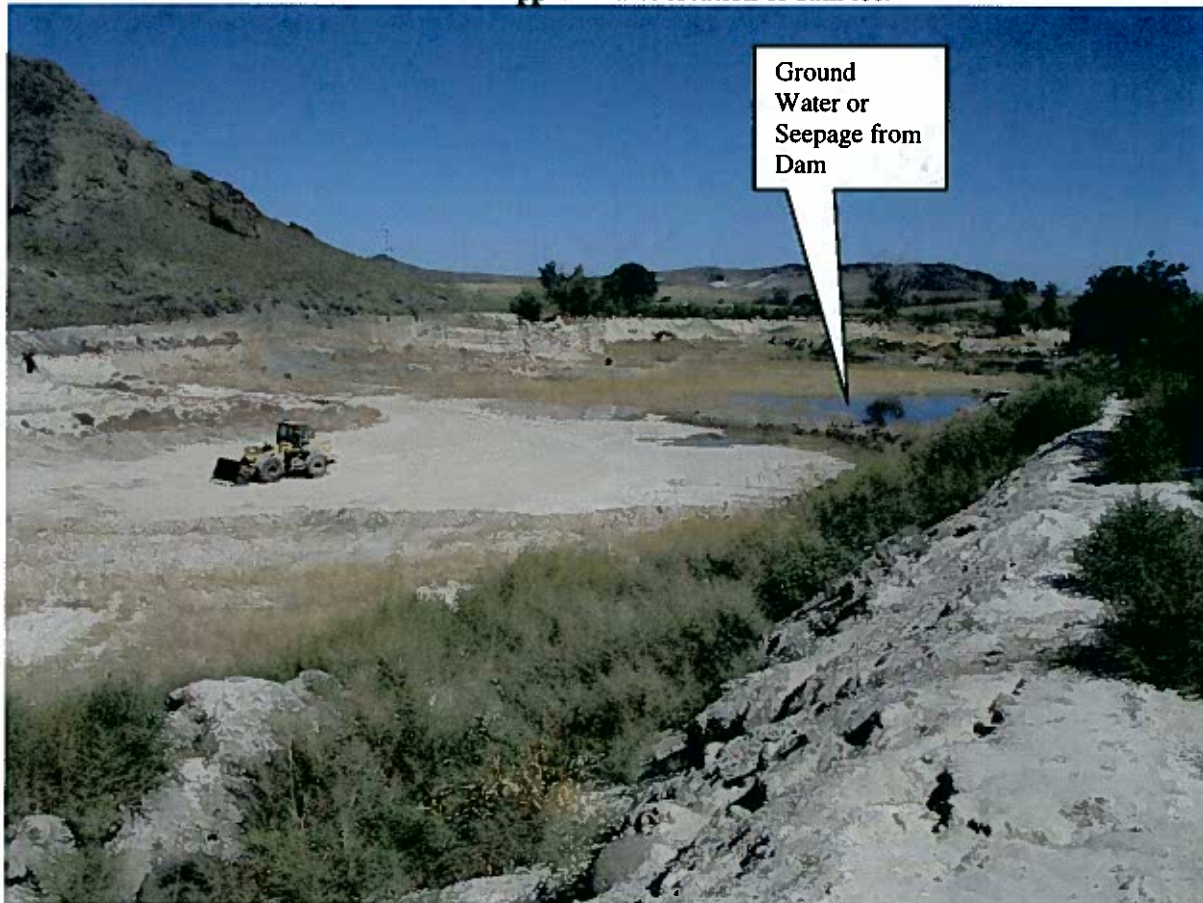
Photo viewing extent of pit as seen from western edge of dam.
