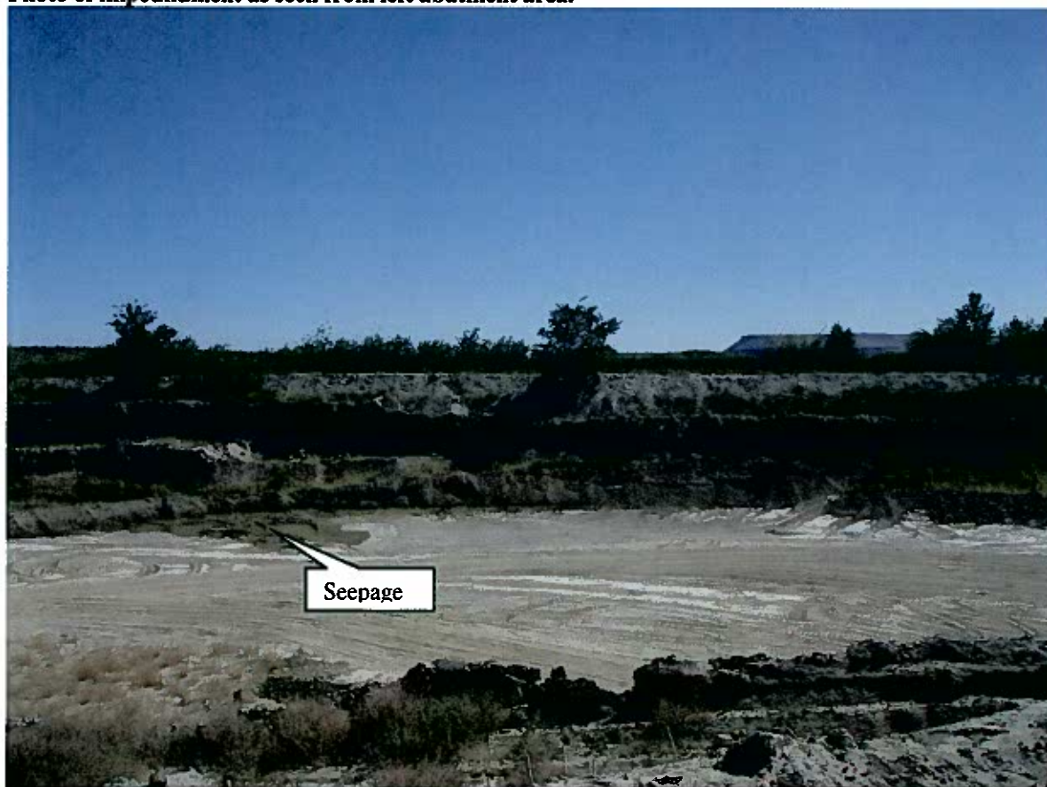
Close-up of pit excavation and downstream face of dam.
