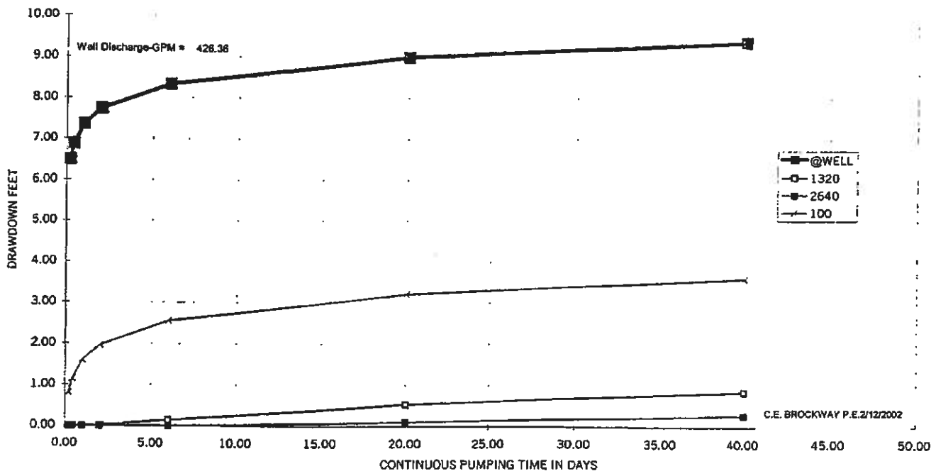
ESTIMATED DRAWDOWN FROM PROPOSED BROOKWOOD EXCHANGE WELL
