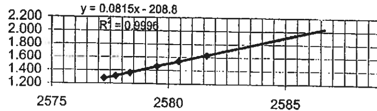
Brookwood Pond No 5 Area vs Elev
