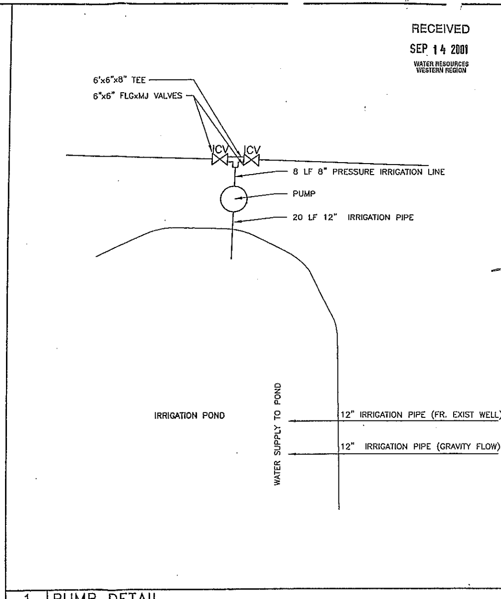
1 PUMP DETAIL
