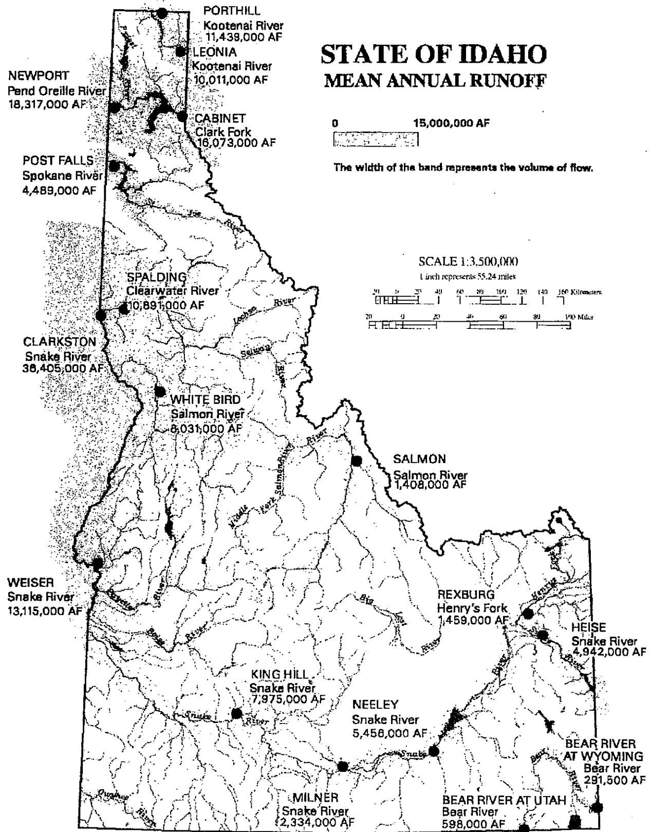
Figure 4. State of Idaho Mean Annual Run-Off
