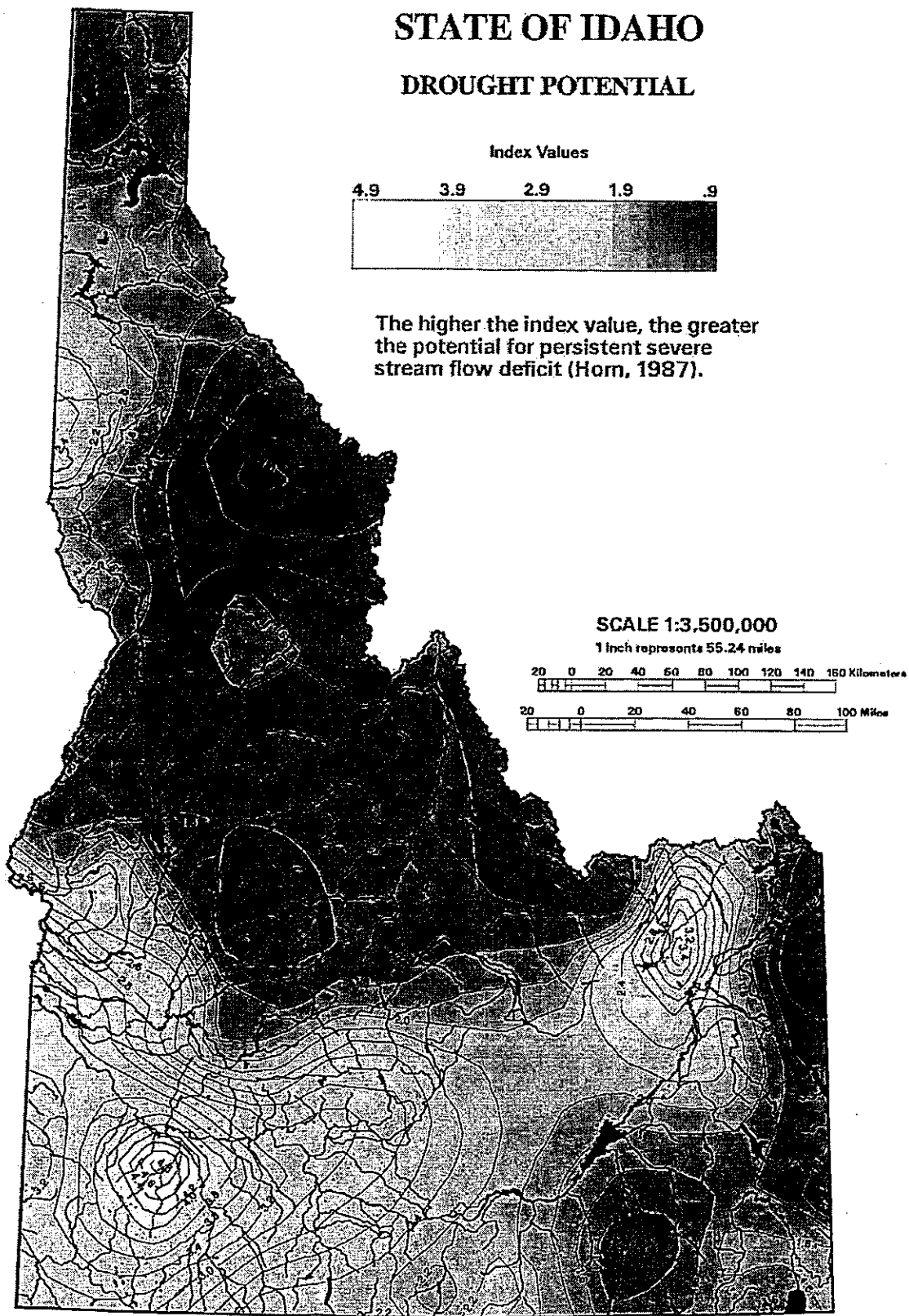
Figure 23. State of Idaho Drought Potential
