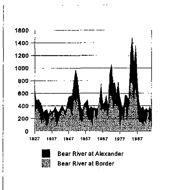
Figure 22. Annual runoff of the Bear River at the Border and Alexander gaging stations, 1927 - 1995. Runoff in thousand acre-feet.
