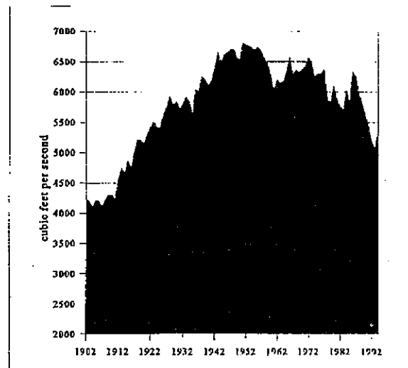
Figure 12. Average annual ground water discharge from the north side of the Snake River between Milner and King Hill. Discharge in cubic-feet per second for years 1902 through 1994.
