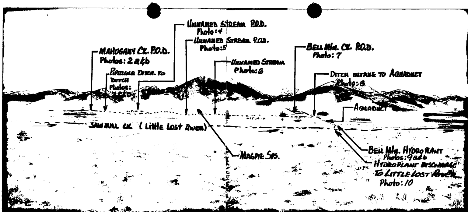
Photo 1. ABOVE - OVERVIEW OF BELL Mtn. HYDRO SYSTEM.
