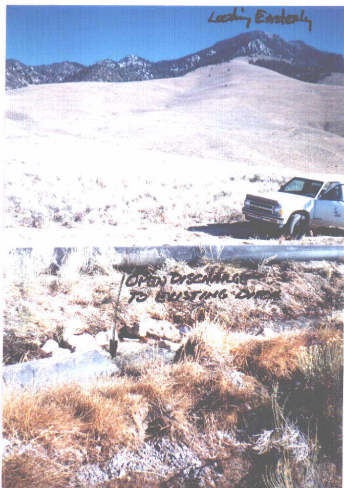
Photo 2d. SHOWS OPEN DISCHARGE OF NEW PIPELINE TO EXISTING DITCH AT SENESW SEC. 30 T. 11N., R. 27E.
