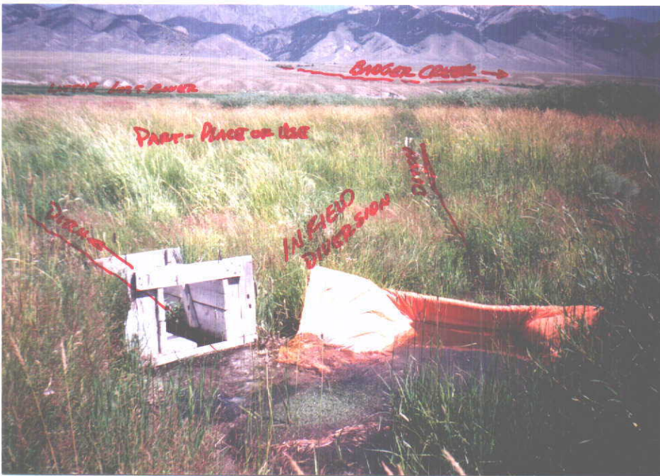
Photo 2. SHOWS DAM & HEADBOX OF IN-FIELD DITCH AND A PORTION OF PLACE OF USE.
