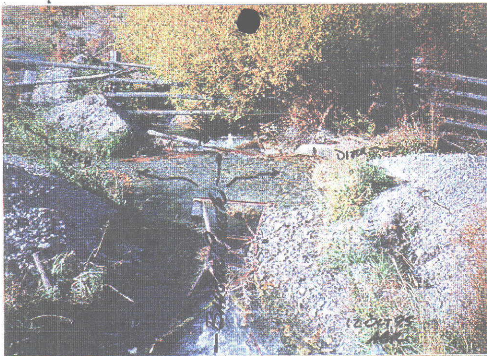
Photo 1. TAKEN FROM THE LITTLE LOST RIVER HIGHWAY AT THE BADGER CREEK CULVERT. THIS IS THE POINT OF DIVERSION FROM BADGER CREEK. AN EXCHANGE DIVERSION FROM THE LITTLE LOST RIVER IS ALSO USED (SEE PHOTO 4 THIS SET) USE OF BADGER CREEK WATER IS EXCHANGED FOR LITTLE LOST RIVER WITH 33-00032 (CLAIMED AS: A33-00032A).
