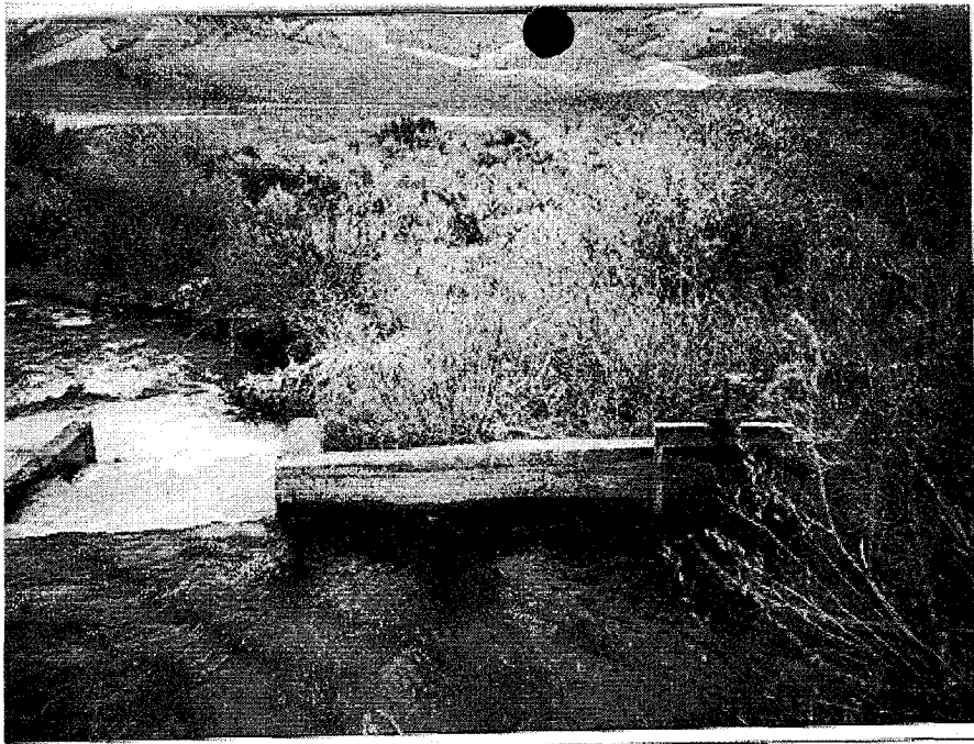
Photo 1. DIVERSION OF WET CK WATERS TO REED PLACE. P.O.D. NENW NE SEC. 5 T. 9N, R. 27E.
