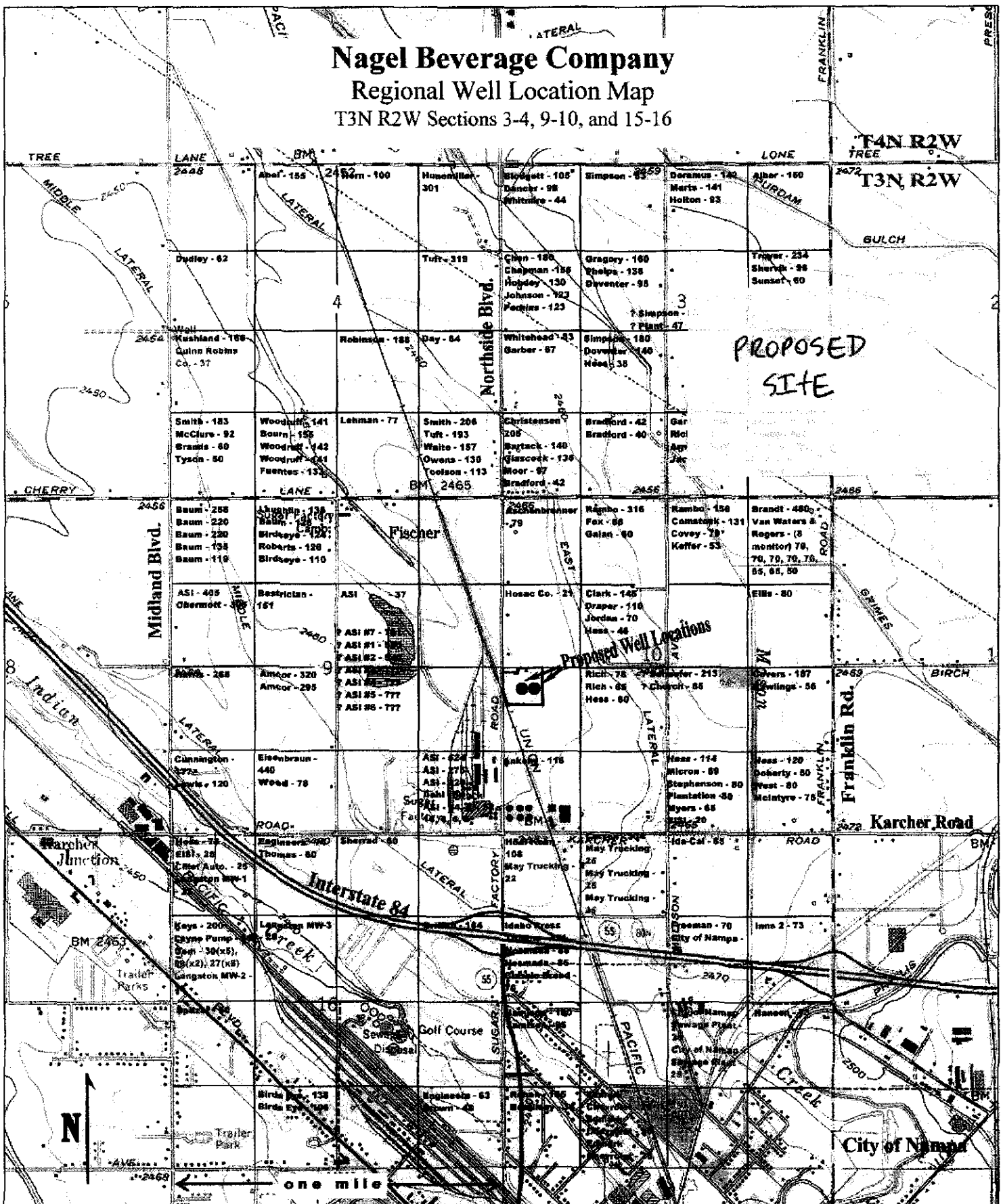
Figure 1. Location map of wells in T3N R2W Sections 3-4, 9-10, and 15-16. Wells are plotted to the nearest 1/4, 1/4 section by name followed by total depth of the well. Owing to space consideration, the five deepest wells are plotted in each 1/4, 1/4 section. If less than five wells exist in a 40-acre tract, then the wells plotted are the only wells listed. Wells in red are monitoring wells and wells in center of section are of unknown location. Some well logs may be missing and others may be mislocated on well log. Map is a 1:24,000 scale USGS 7 1/2 -
