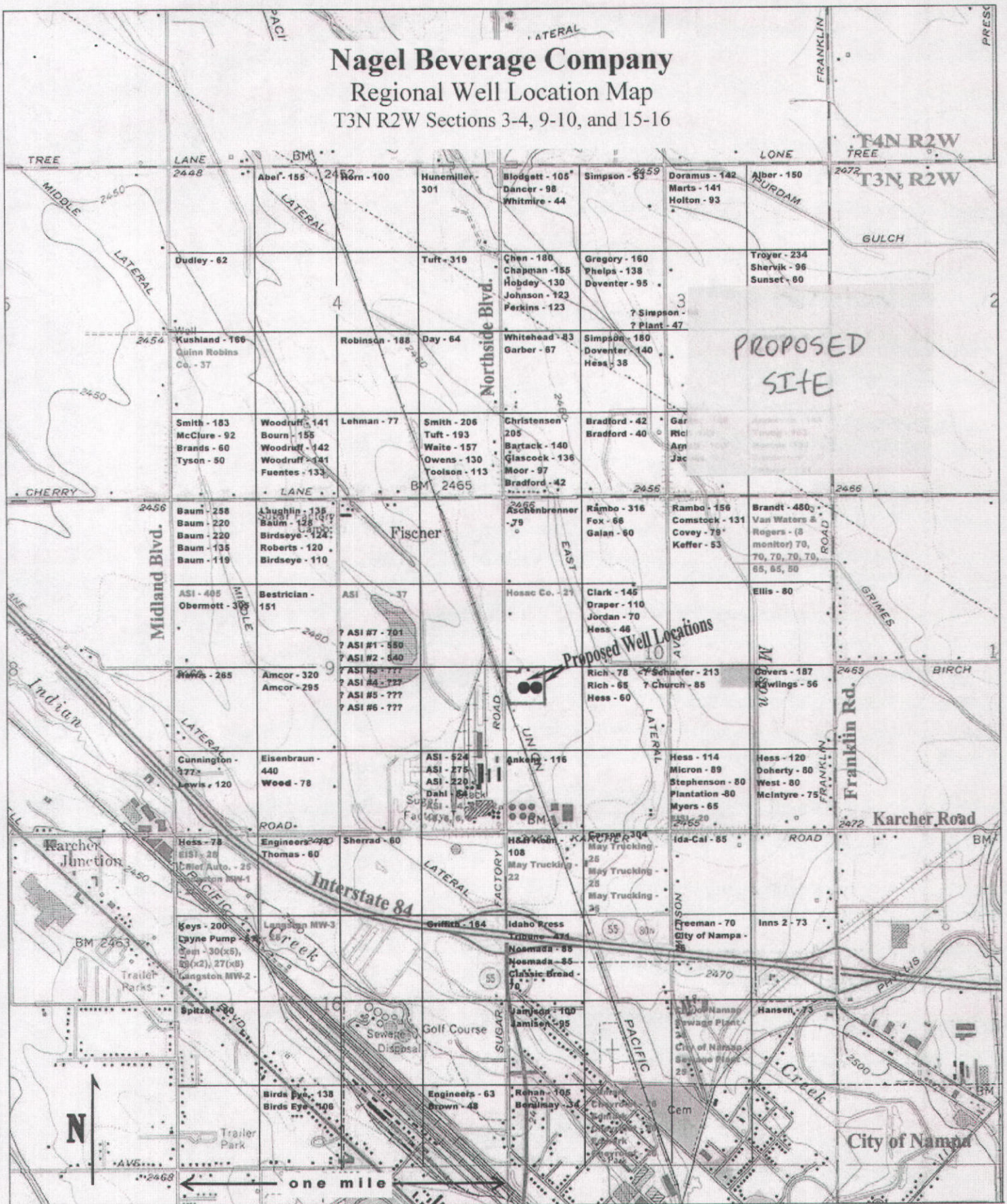
Figure 1. Location map of wells in T3N R2W Sections 3-4, 9-10, and 15-16. Wells are plotted to the nearest \frac{1}{4} , \frac{1}{4} section by name followed by total depth of the well. Owing to space consideration, the five deepest wells are plotted in each \frac{1}{4} , \frac{1}{4} section. If less than five wells exist in a 40-acre tract, then the wells plotted are the only wells listed. Wells in red are monitoring wells and wells in center of section are of unknown location. Some well logs may be missing and others may be mislocated on well log. Map is a 1:24,000 scale USGS 7 \frac{1}{2} -
