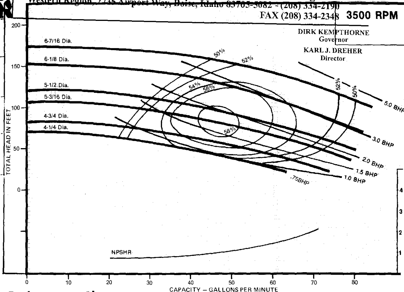
Performance Chart - 3500RPM
