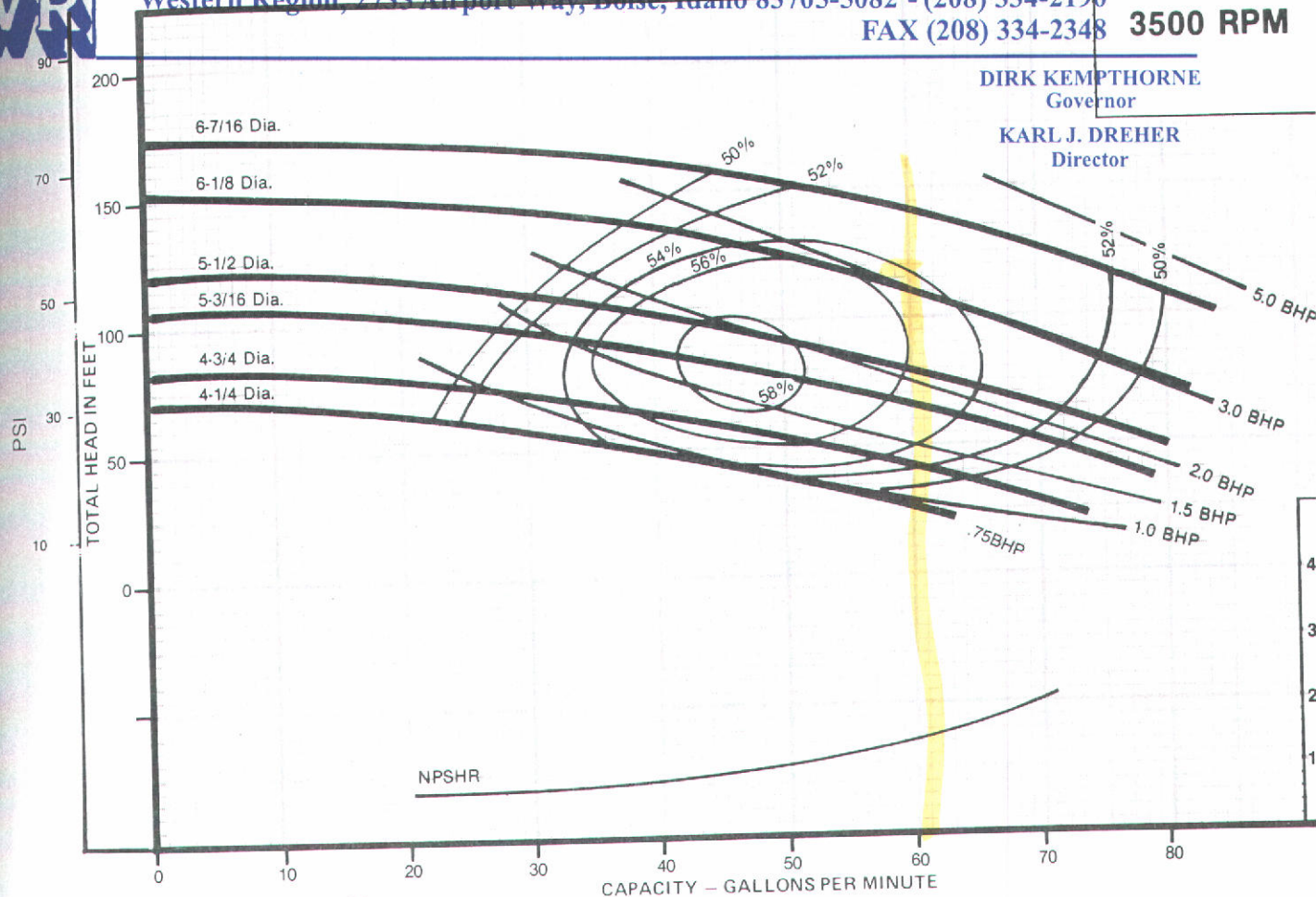
Performance Chart - 3500RPM
