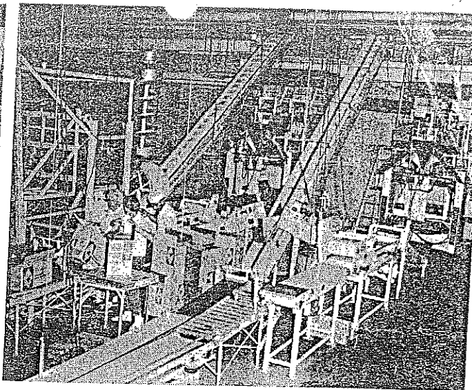
Automatic packaging of institutional French fries in Tite-pak bags reach final stage prior to shipping
