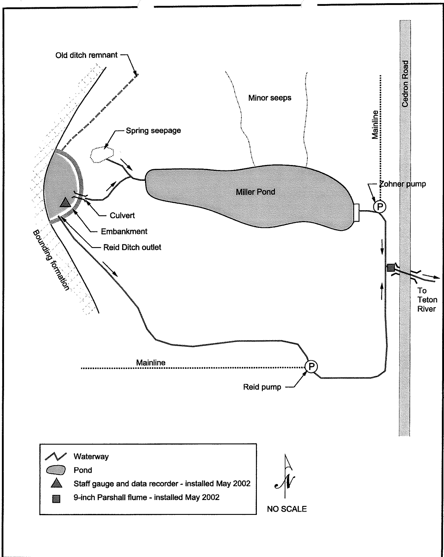
Figure 2. Diagram of the Paradise Spring collection and distribution system.
