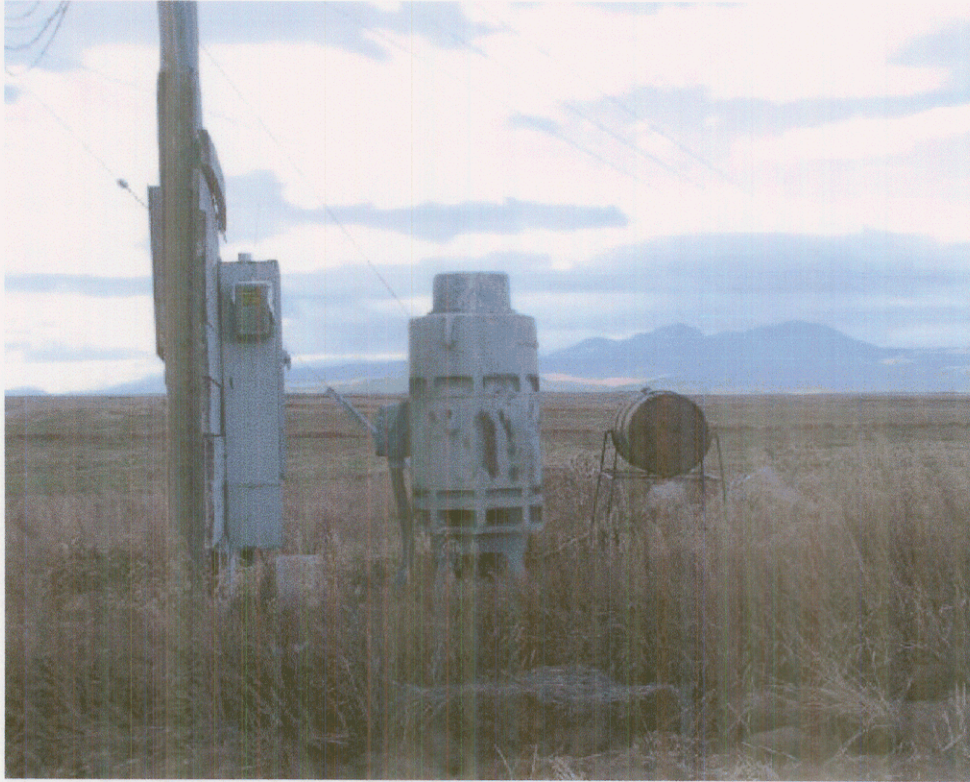
Photo 1. G.E. 125 hp pump, Model 5K505XC024A. Looking northeasterly. (IMG_0182.JPG)
