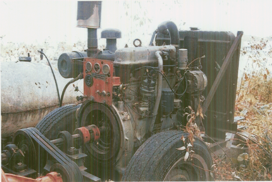
Looking west. Mobil Diesel powered pump. HP – Unknown: Model – VRG155: Size 3/ 8x3 3 / 4 . White tank is the fuel tank. Pocatello creek behind me in the picture (csaxton 10/25/01).
