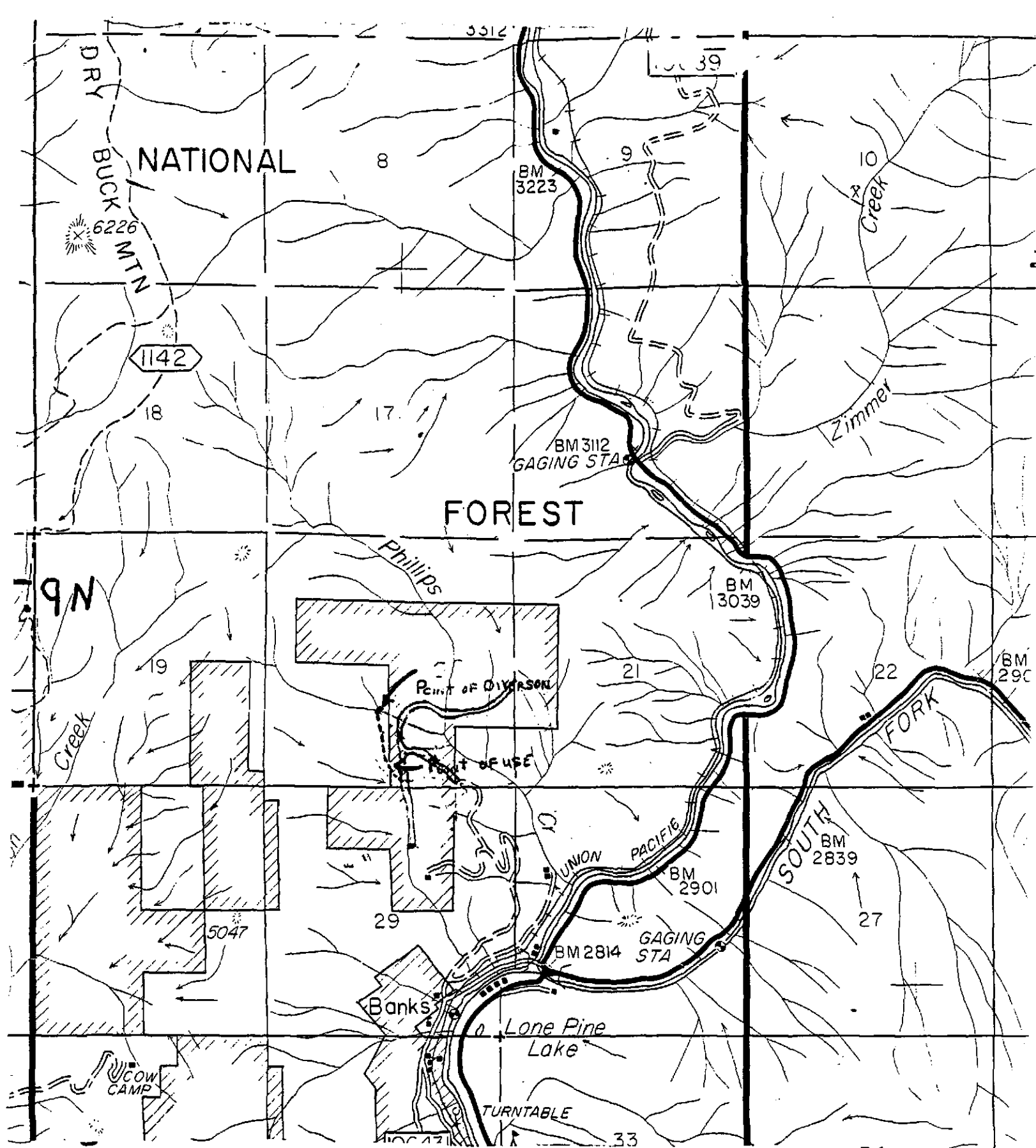
WATER DIVERSION AND TRANSMISSION LINE EMERY AND MARCIA SMITH SW1/4 Section 20, T.9N., R.3E.
