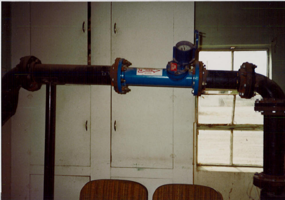
Well meter on well dating from the 1940's. Well is housed in shop behind Homedale City Hall.
