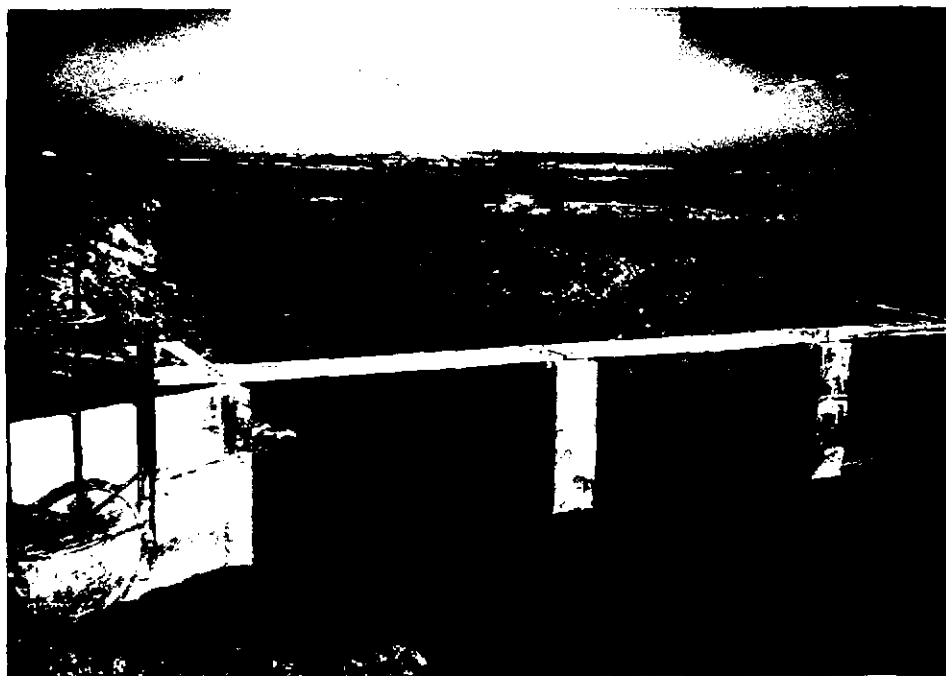
JUMP CK. DIVER- SION LOOKING DOWN- STREAM FACING (NORTH) WITH HEADGATE ON LEFT SIDE OF PHOTO.
