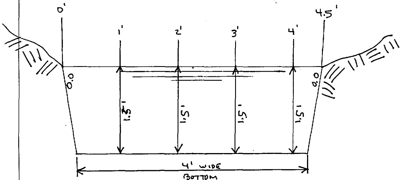
X-SEC DIMENSIONS FOR DITCH FROM TINDALL RESERVOIR.
