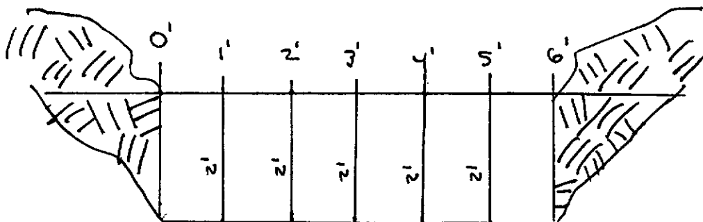
CANAL RATTLESNAKE X-SECTION
