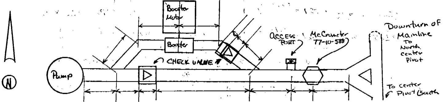
SCHEMATIC DIAGRAM OF SYSTEM
