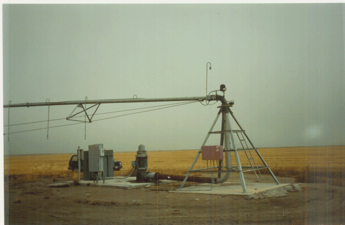
Looking north at well, pump & pivot tower from approximately 50 ft. south of well.
