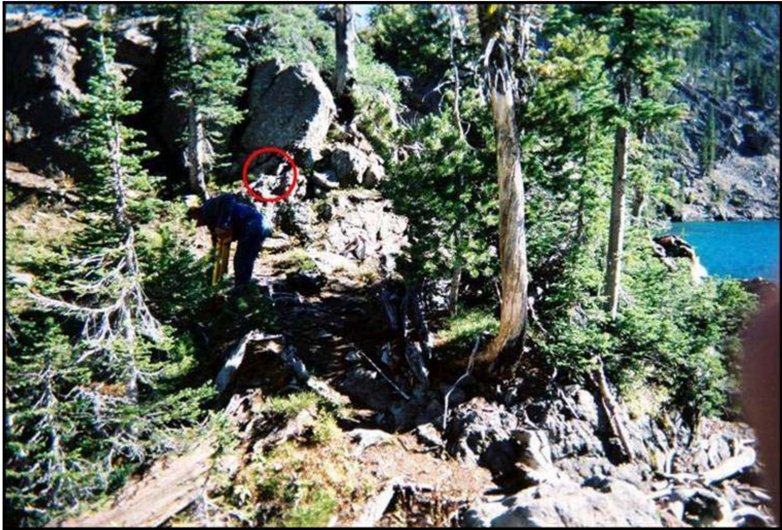
BM-1, Aluminum benchmark drilled and driven into rock, then covered with soil and rocks to hide the cap (inside circle).
