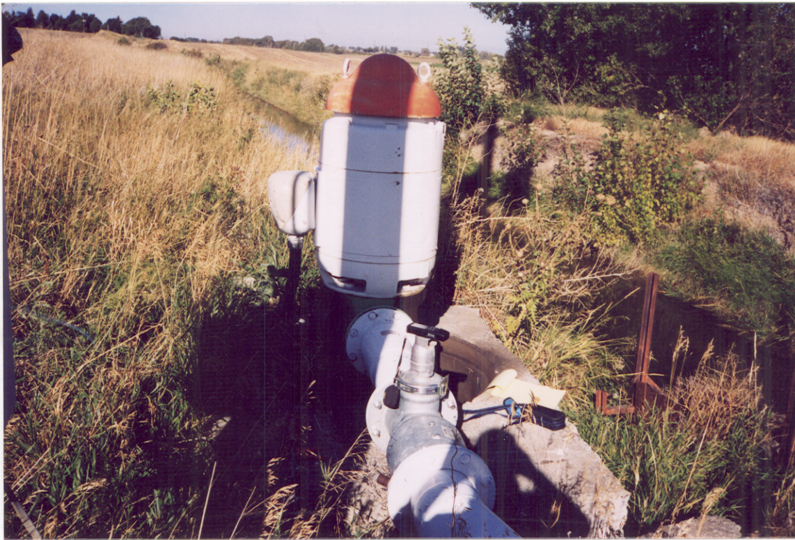
FARMER'S FRIEND Canal pump
