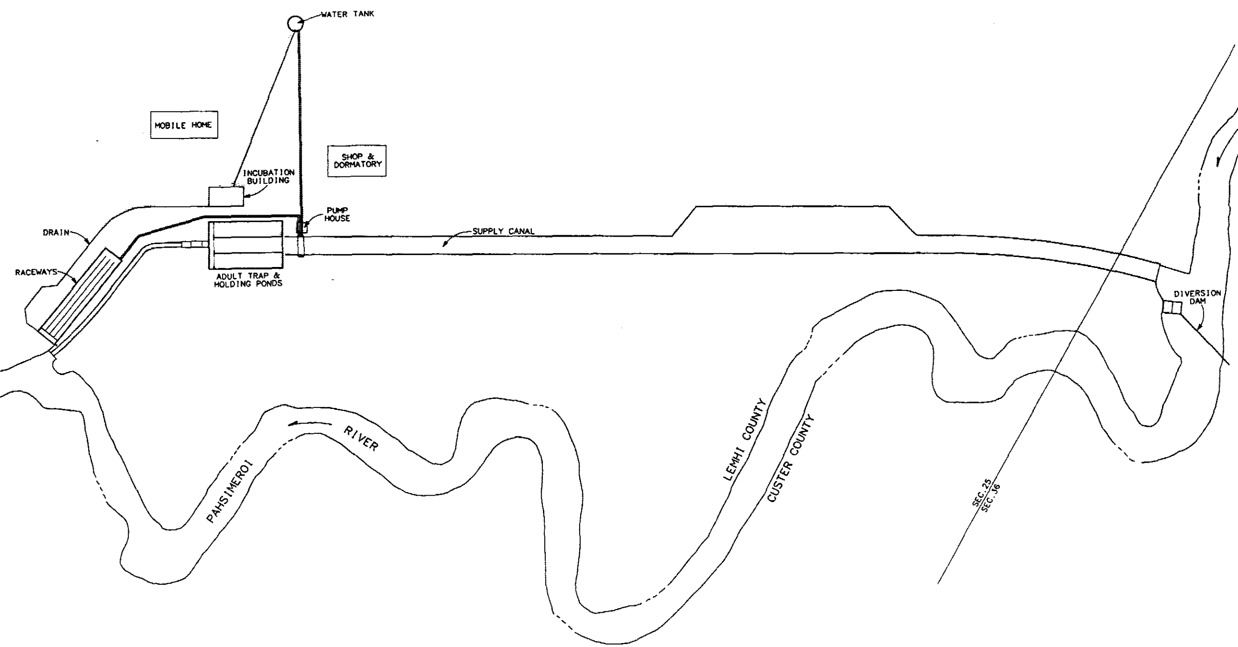
FUNCTIONAL DRAWING WATER RIGHT A 73-07055 FOR 40.0 CFS PAHSIMEROI RIVER STEELHEAD HOLDING PONDS & EYEING STATION LEMHI CO., IDAHO
